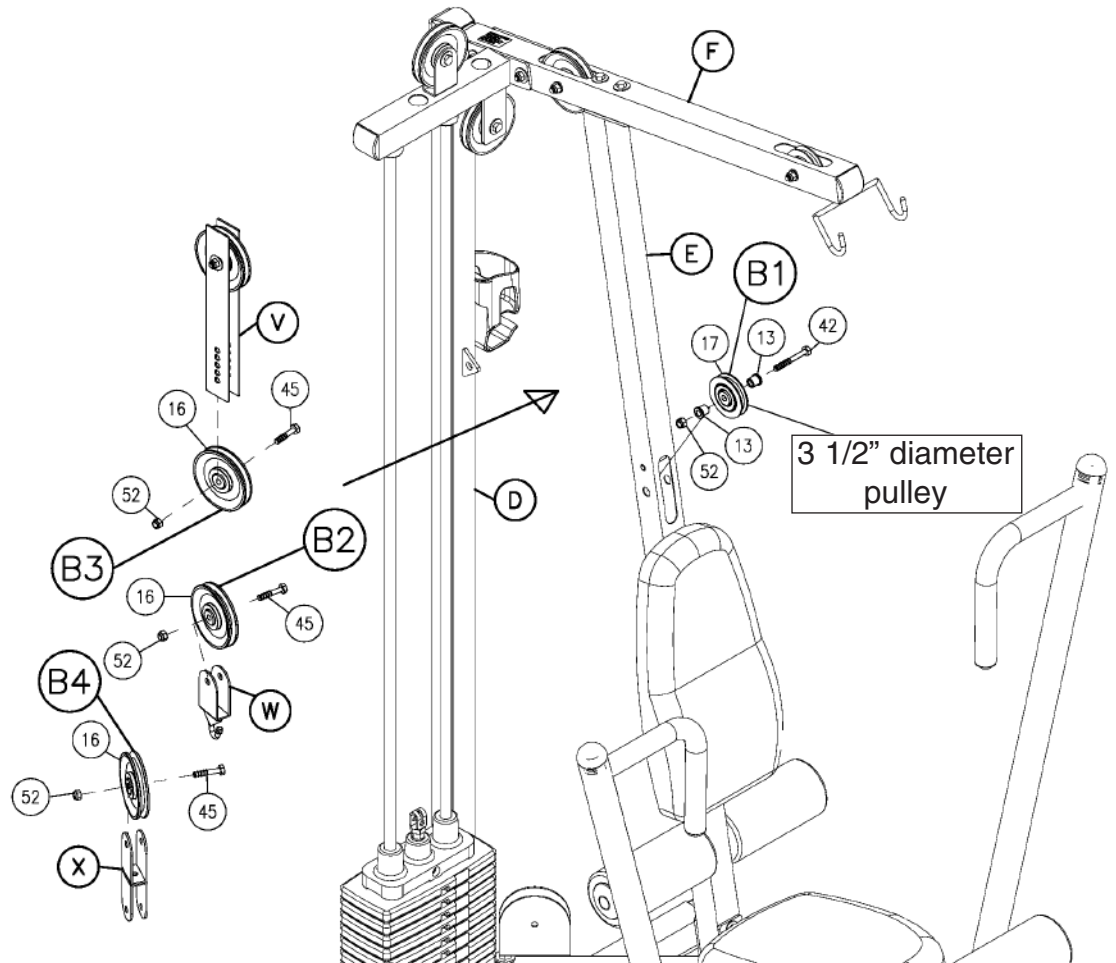
Diagram 2 Pulley Installation
