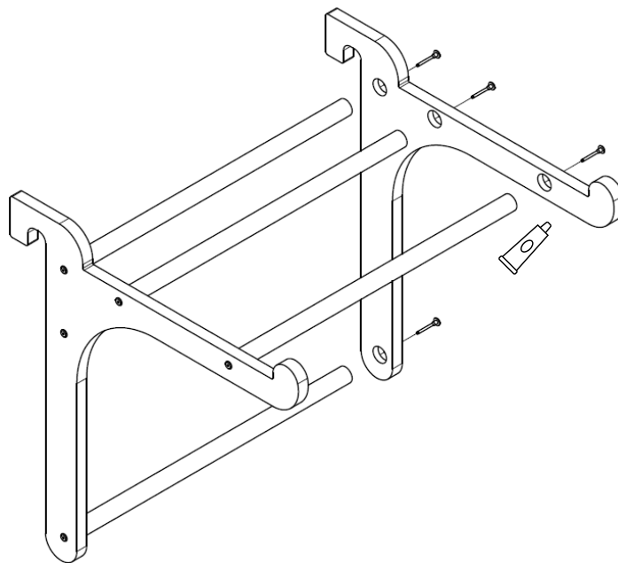
Figure 4: Assembly – right side panel
