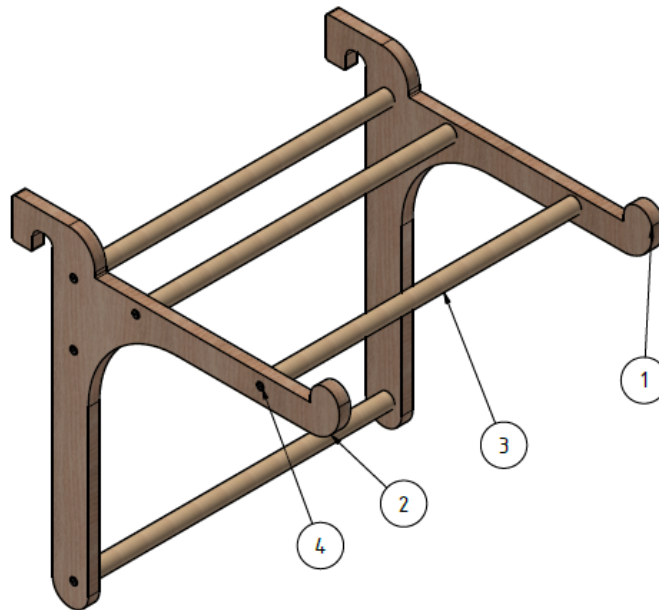
Figure 2: Pull-up bar "Wood"
